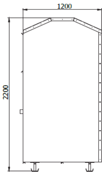
StorePartner KS z dachem dwuspadowym StorePartner KS with gable roof
