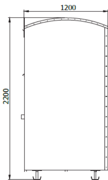
StorePartner KS z dachem okrągłym StorePartner KS with rounded roof
