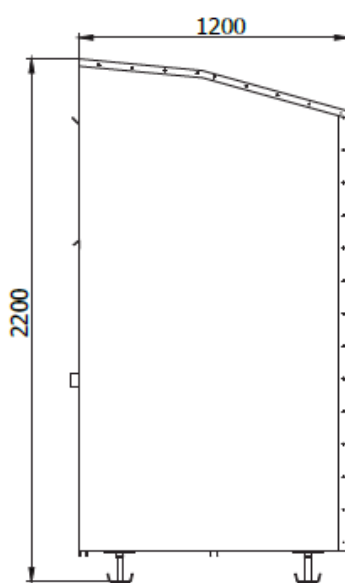
StorePartner KS z dachem dwuspadowym StorePartner KS with flat slanted roof
